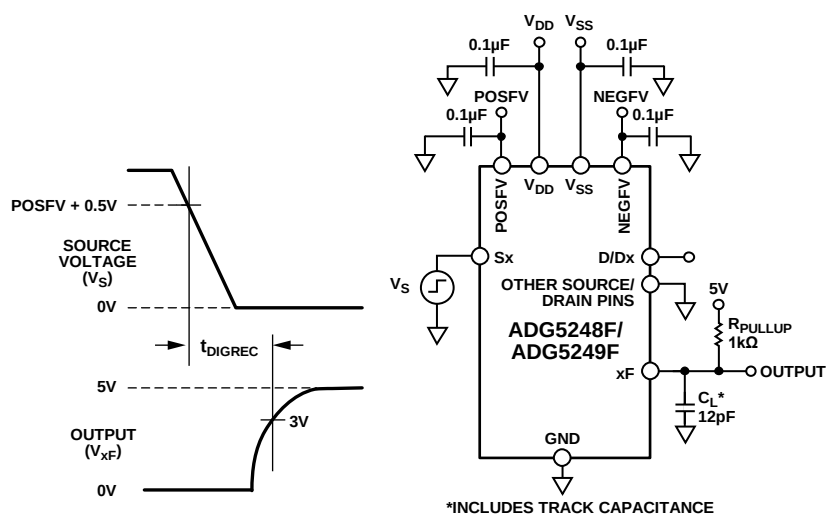
Figure 45. Interrupt Flag Recovery Time, t_{DIGREC} , with a 1\text{ k}\Omega Pull-Up Resistor
