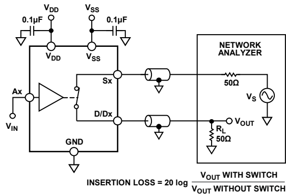
Figure 40. Bandwidth
