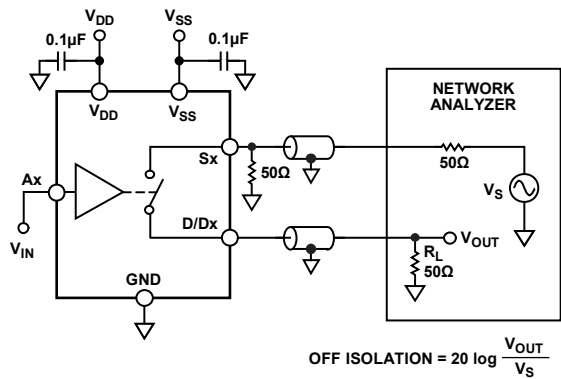
Figure 39. Off Isolation
