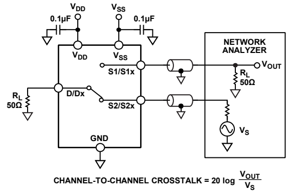
Figure 38. Channel-to-Channel Crosstalk
