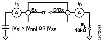
Figure 33. Switch Overvoltage Leakage
