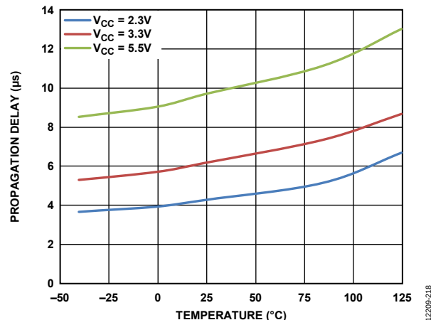
Figure 18. Propagation Delay vs. Temperature, High to Low, V_{OD} = 10mV
