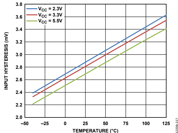
Figure 17. Input Hysteresis vs. Temperature, V_{CM} = 1V for Various Supply Voltages ( V_{CC} )
