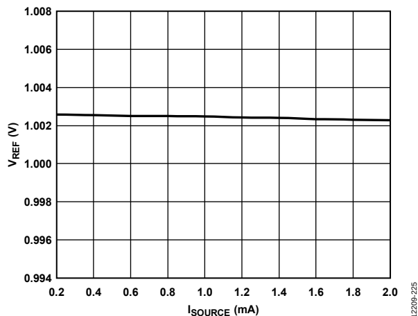
Figure 25. Reference Voltage ( V_{REF} ) vs. Source Current ( I_{SOURCE} ) of the REF Pin, V_{CC} = 3.3 V
