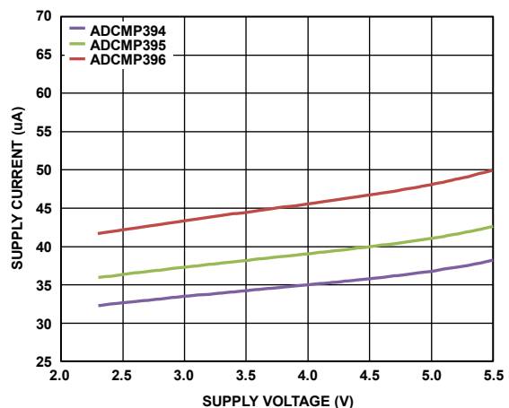
Figure 12. Supply Current ( I_{CC} ) vs. Supply Voltage ( V_{CC} ) at Output High Voltage
