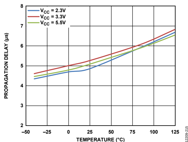
Figure 15. Propagation Delay vs. Temperature, Low to High, V_{OD} = 10mV
