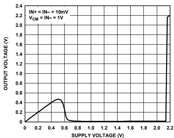
Figure 11. Output Voltage ( V_{OUT} ) vs. Supply Voltage ( V_{CC} ), R_{PULLUP} = 10\text{ k}\Omega
