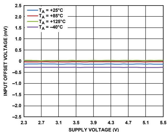
Figure 10. Input Offset Voltage ( V_{OS} ) vs. Supply Voltage ( V_{CC} ), V_{CM} = 1\text{ V} for Various Temperatures
