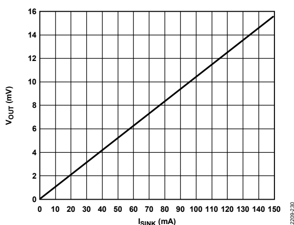
Figure 30. Output Voltage ( V_{OUT} ) Low vs. Sink Current ( I_{SINK} ), V_{CC} = 0.9 V
