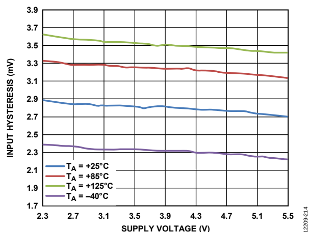
Figure 14. Input Hysteresis vs. Supply Voltage ( V_{CC} ), V_{CM} = 1V for Various Temperatures
