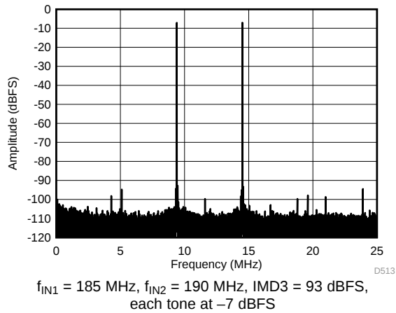
Figure 44. FFT for Two-Tone Input Signal ( -7\text{ dBFS} at 185 MHz and 190 MHz)
