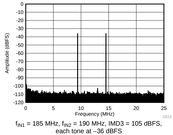
Figure 45. FFT for Two-Tone Input Signal ( -36\text{ dBFS} at 185 MHz and 190 MHz)
