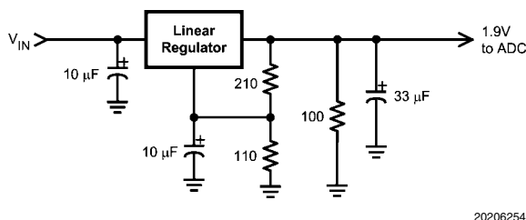
FIGURE 16. Non-Spiking Power Supply
