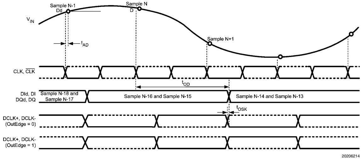
FIGURE 3. ADC08D1020 Timing — SDR Clcking in 1:2 Demultiplexed Mode
