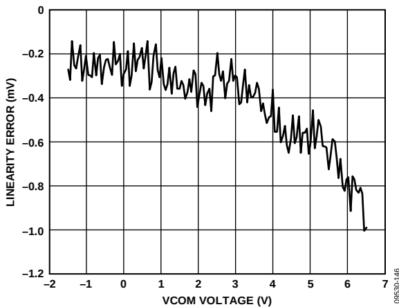
Figure 53. Active Load VCOM Linearity Error
