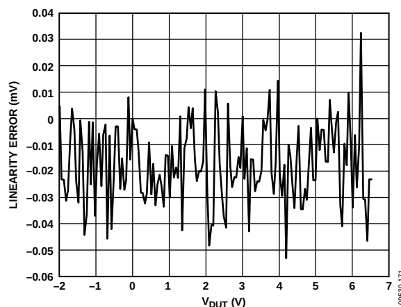
Figure 78. PPMU Range B Measure Voltage Linearity Error
