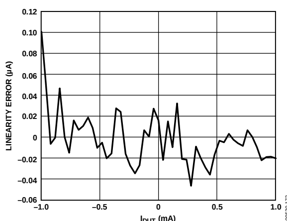
Figure 79. PPMU Range B Measure Current Linearity Error
