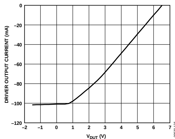
Figure 32. Driver Output Current Limit. Driver Programmed to 6.5 V, V_{OUT} Swept -1.5 V to +6.5 V
