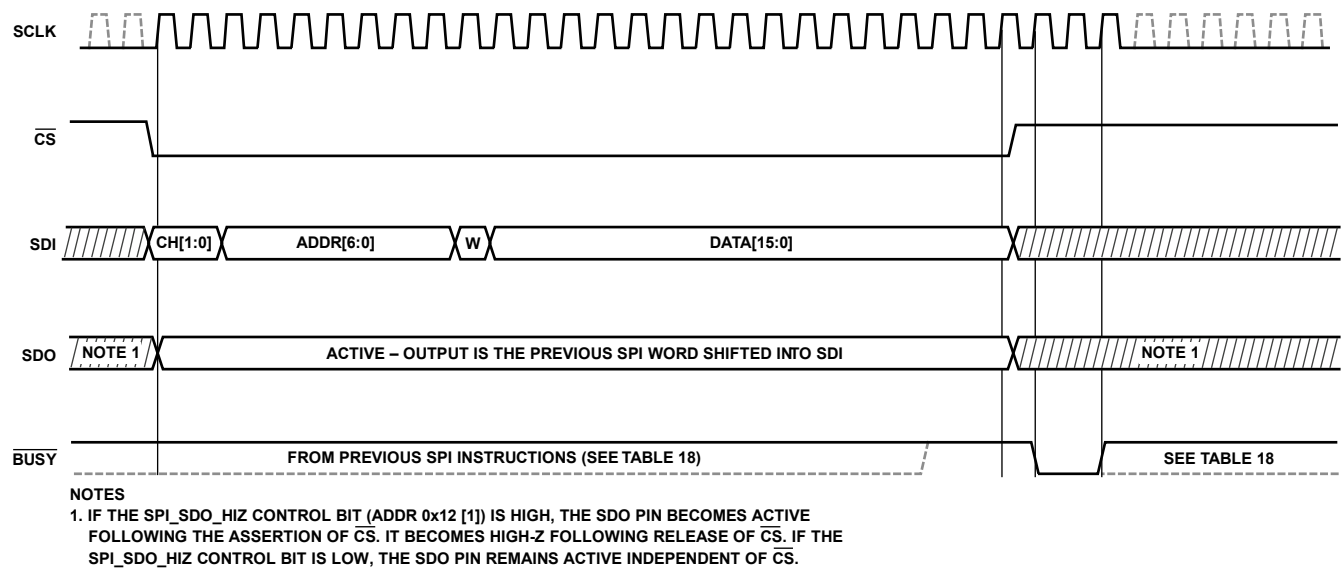
Figure 3. SPI Write Instruction
