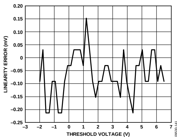
Figure 48. PPMU Go/No-Go Comparator Linearity Error
