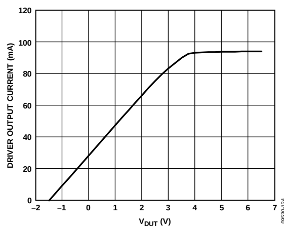
Figure 31. Driver Output Current Limit; Driver Programmed to -1.5 V, V_{OUT} Swept -1.5 V to +6.5 V
