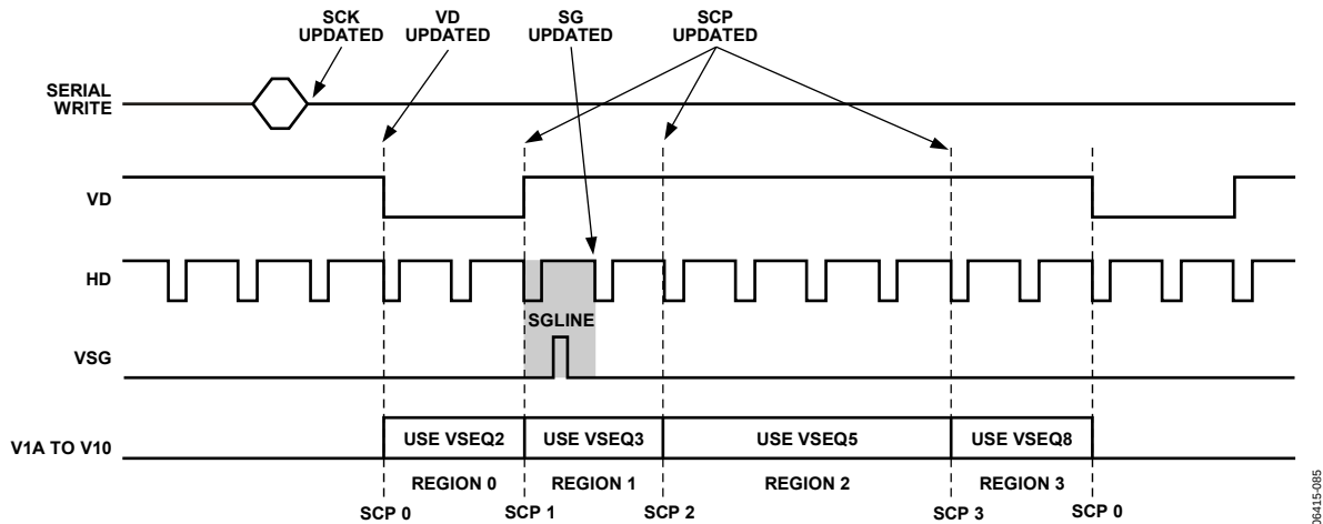
Figure 88. Register Update Locations (See Table 44 for Definitions)
