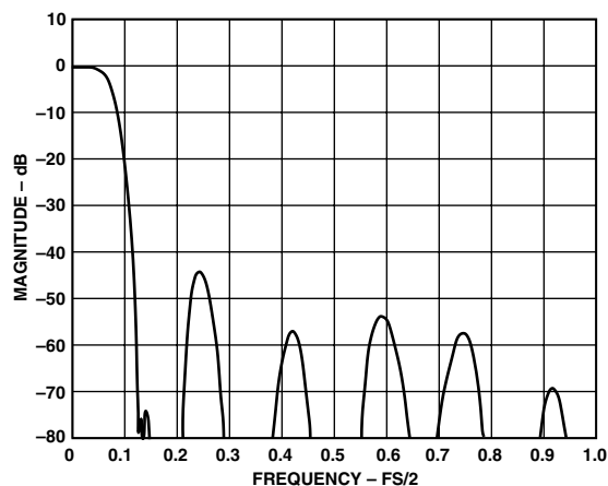
Figure 11a. Cascaded Filter 16 \times Interpolator ( N = 4 )
