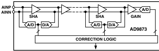
Figure 17. ADC Architecture
