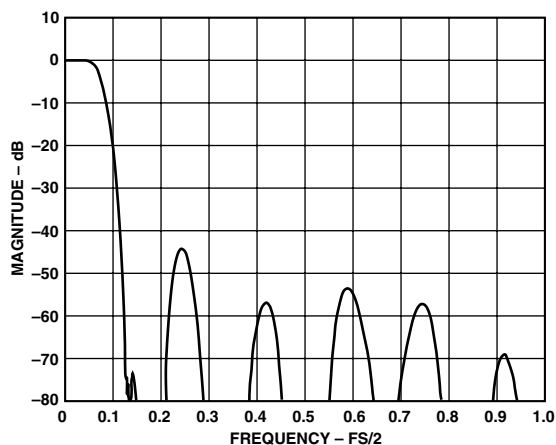
Figure 10a. Cascaded Filter 12 \times Interpolator ( N = 3 )
