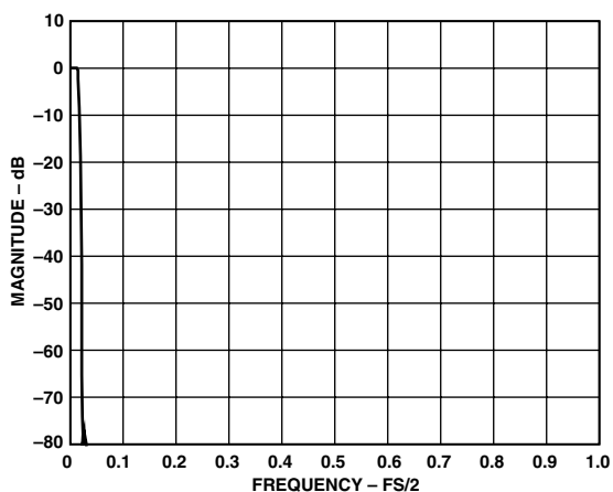
Figure 10c. Response to Input Signal Spectrum ( N = 3 )
