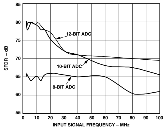
TPC 18. SFDR vs. Input Frequency
