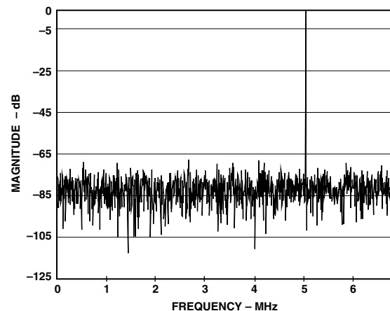
TPC 20. 8-Bit ADC Single-Tone Spectral Plot Using PLL (Input Frequency = 5 MHz, 2048 Point FFT)
