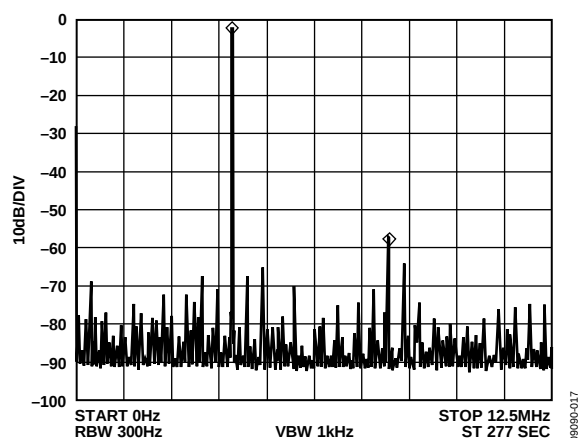
Figure 17. f_{MCLK} = 25 MHz, f_{OUT} = 4.1 MHz, Frequency Word = 0x29FBE76D
