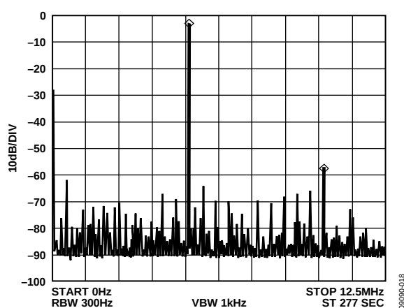
Figure 18. f_{MCLK} = 25 MHz, f_{OUT} = 5.1 MHz, Frequency Word = 0x34395810
