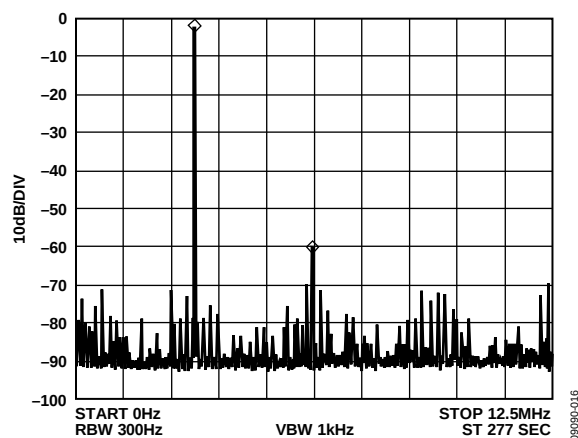
Figure 16. f_{MCLK} = 25 MHz, f_{OUT} = 3.1 MHz, Frequency Word = 0x1FBE76C9
