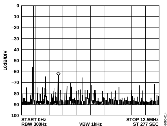
Figure 14. f_{MCLK} = 25 MHz, f_{OUT} = 1.1 MHz, Frequency Word = 0xB439581
