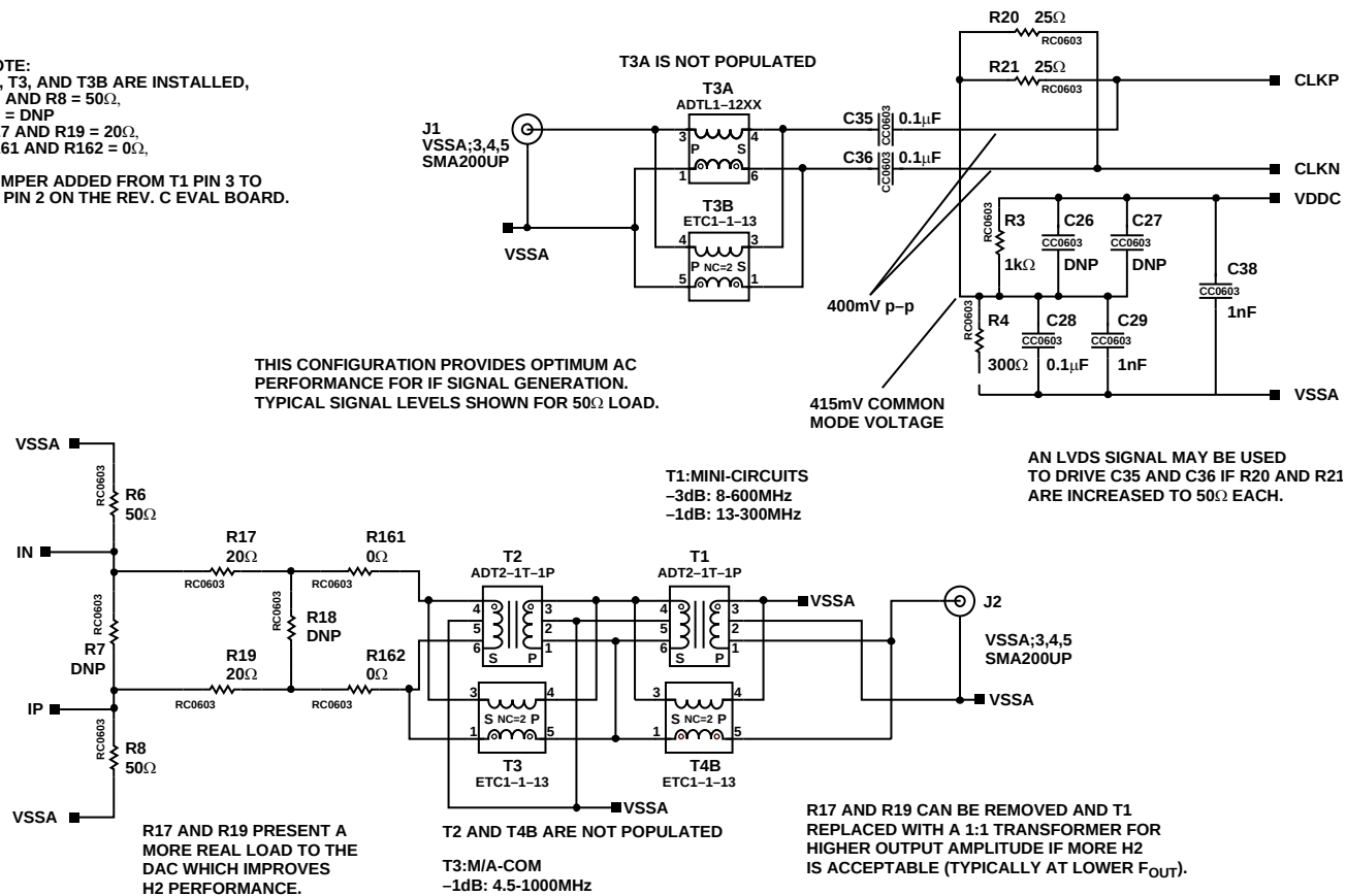
Figure 107. Clock Input and Analog Output, AD973x Evaluation Board, Rev. F
