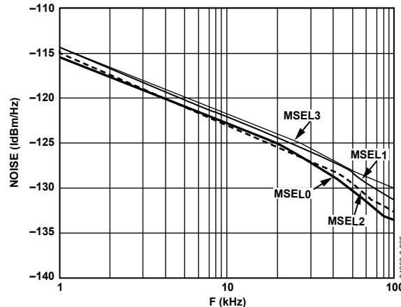
Figure 87. 1/f Noise with Respect to MSEL Bits
