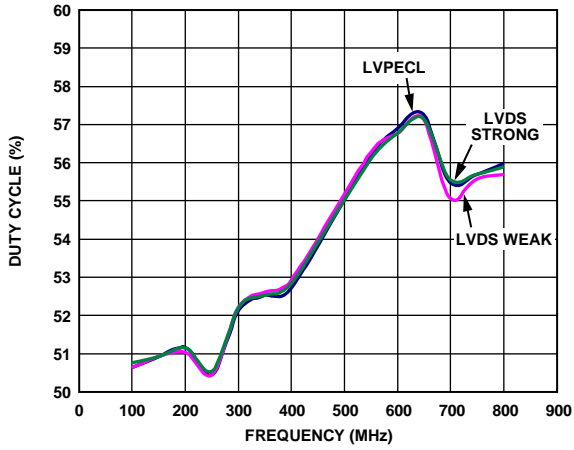
Figure 15. Duty Cycle vs. Output Frequency, LVPECL and LVDS (100 \Omega Load)
