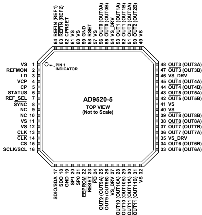
Figure 5. Pin Configuration
