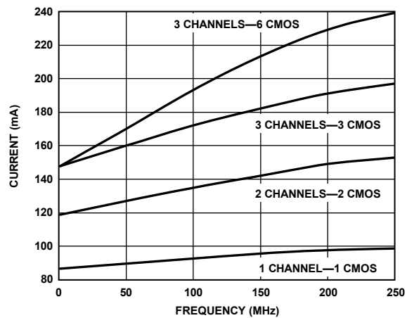
Figure 7. Total Current vs. Frequency, CLK-to-Output (PLL Off), CMOS Outputs with 10\text{ pF} Load
