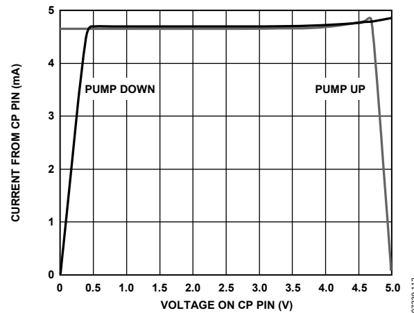
Figure 9. Charge Pump Characteristics at C_P = 5.0\text{ V}
