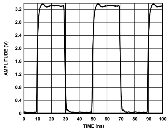
Figure 15. CMOS Output with 10 pF Load at 25 MHz
