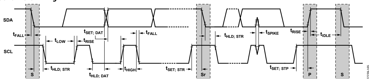
Figure 49. I 2 C Serial Port Timing
