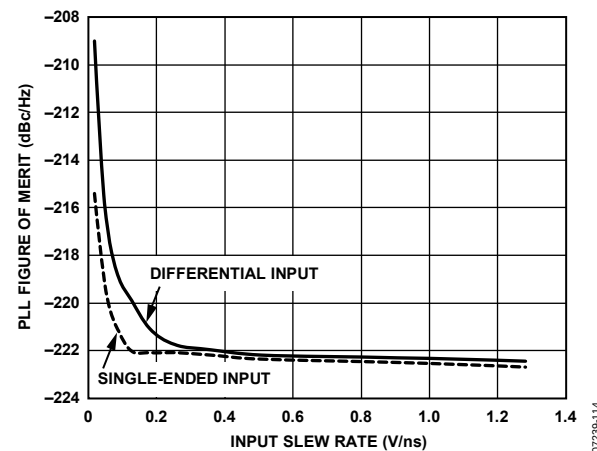
Figure 11. PLL Figure of Merit (FOM) vs. Slew Rate at \overline{\text{REF}}_{\text{IN}}/\overline{\text{REF}}_{\text{IN}}
