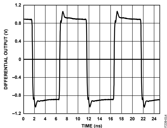
Figure 13. LVPECL Output (Differential) at 100 MHz
