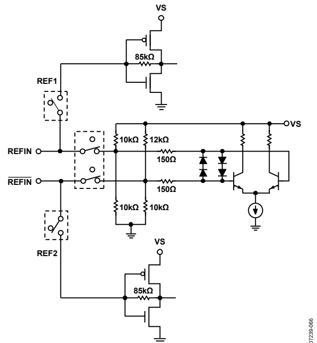
Figure 31. REF1N Equivalent Circuit for Non-XTAL Mode
