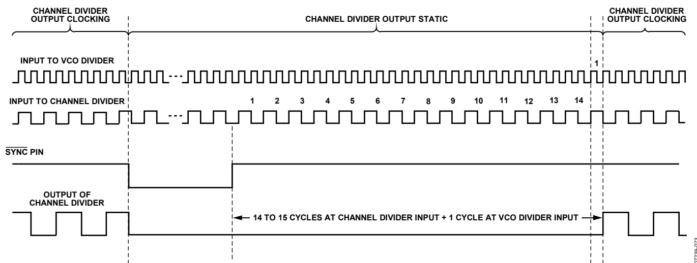
Figure 40. SYNC Timing Pipeline Delay When the VCO Divider Is Used
