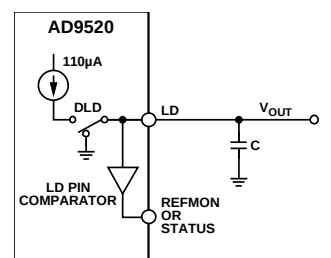
Figure 45. Current Source Digital Lock Detect
