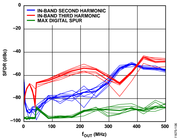
Figure 6. Single-Tone Second and Third Harmonics and Maximum Digital Spur in the First Nyquist Zone, f_{DAC} = 1966\text{ MHz} , 0 dB Back Off
