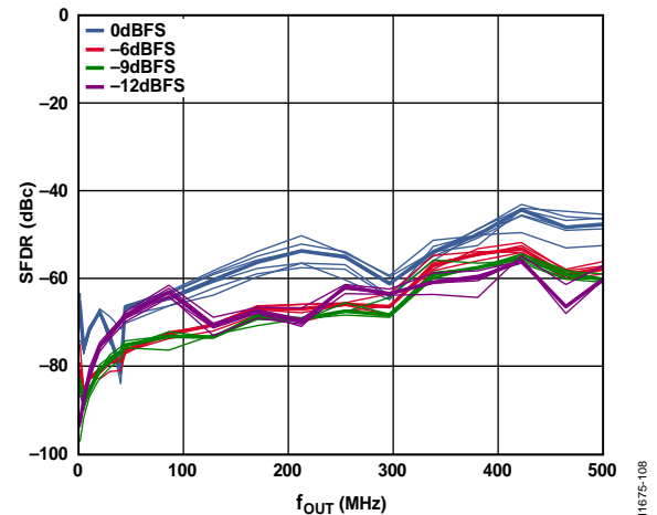
Figure 8. Single-Tone SFDR vs. f_{OUT} in the First Nyquist Zone over Digital Back Off, f_{DAC} = 1966\text{ MHz}
