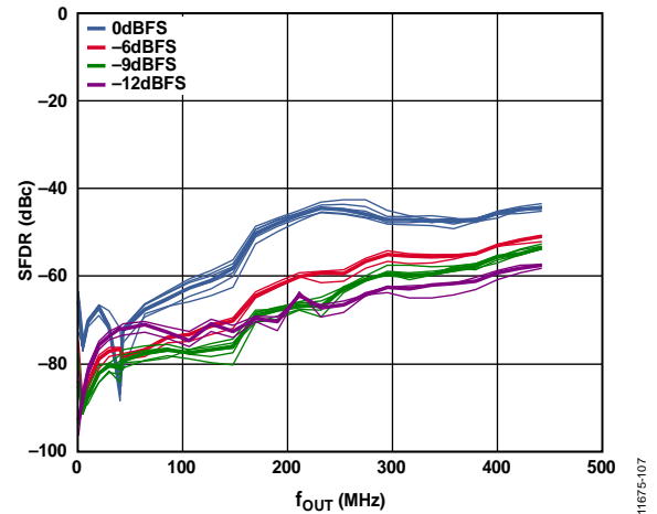
Figure 7. Single-Tone SFDR vs. f_{OUT} in the First Nyquist Zone over Digital Back Off, f_{DAC} = 983\text{ MHz}
