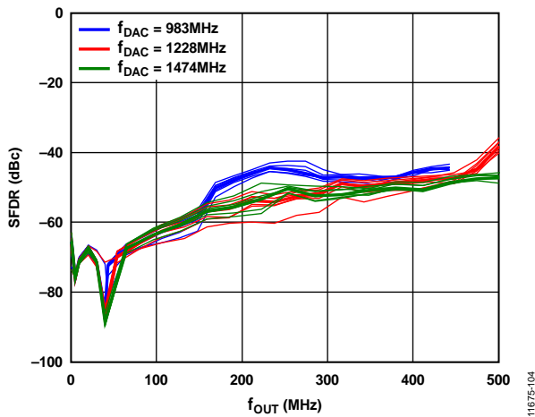
Figure 4. Single-Tone SFDR vs. f_{OUT} in the First Nyquist Zone, f_{DAC} = 983\text{ MHz} , 1228\text{ MHz} , and 1474\text{ MHz}
