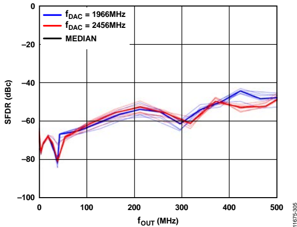
Figure 5. Single-Tone SFDR vs. f_{OUT} in the First Nyquist Zone, f_{DAC} = 1966\text{ MHz} and 2456\text{ MHz}
