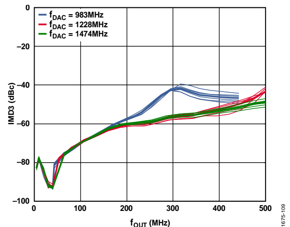
Figure 9. Two-Tone Third IMD (IMD3) vs. f_{OUT} , f_{DAC} = 983\text{ MHz} , 1228\text{ MHz} , and 1474\text{ MHz}
