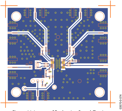
Figure 66. Layout of Evaluation Board, Top Layer
