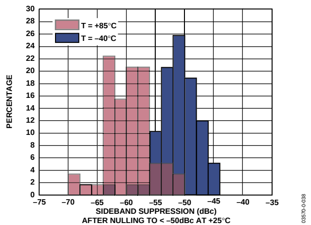
Figure 41. Sideband Suppression Distribution at Temperature Extremes, After Sideband Suppression Nulled to < -50 dBc at T_A = 25^\circ\text{C} . ( F_{LO} = 2140 MHz, F_{BB} = 1 MHz, I and Q Inputs biased at 0.4 V)
