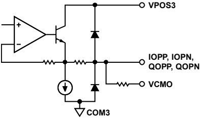
Figure 4. Circuit B
