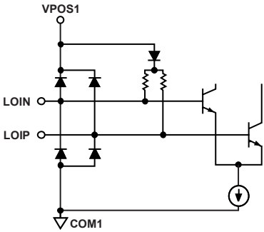
Figure 3. Circuit A
