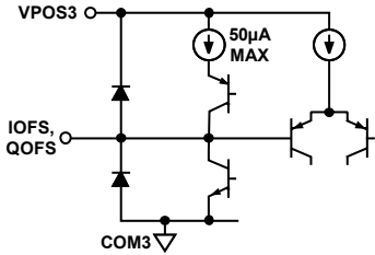
Figure 8. Circuit F
