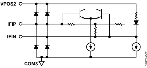
Figure 7. Circuit E
