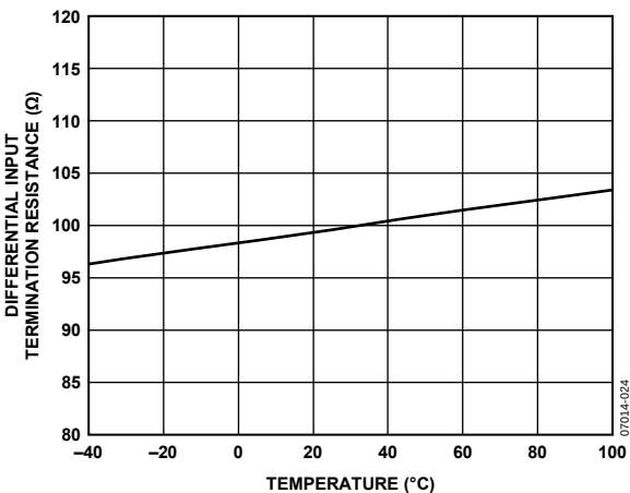
Figure 24. Differential Input Termination Resistance vs. Temperature
