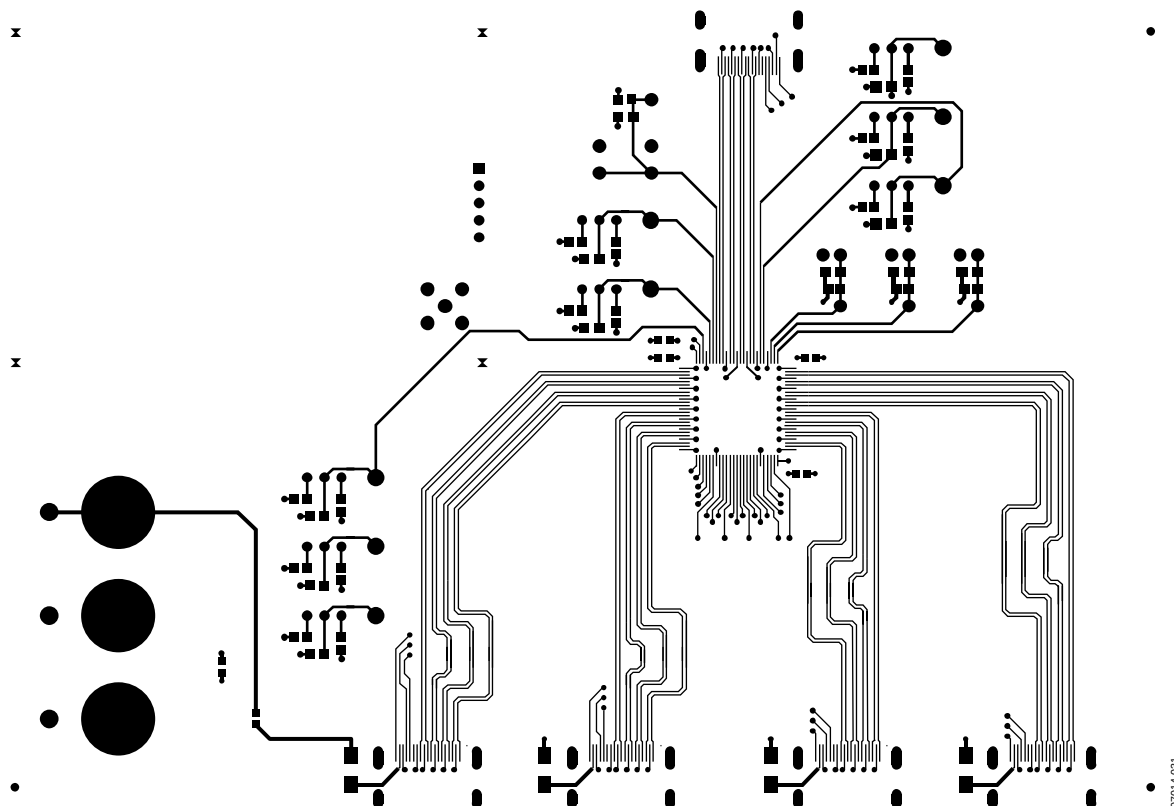
Figure 31. Layout of the TMDS Traces on the AD8197A Evaluation Board (Only Top Signal Routing Layer is Shown)
