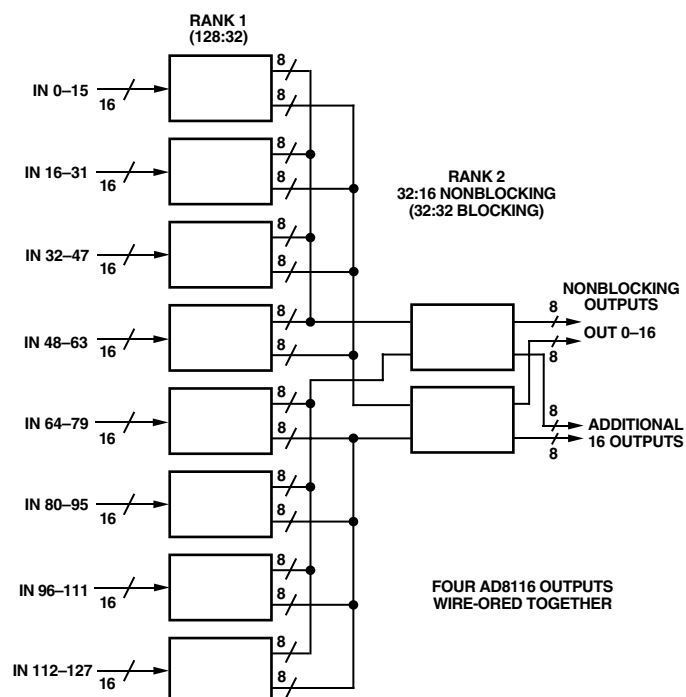
Figure 8. Nonblocking 128 \times 16 Array ( 128 \times 32 Blocking)
