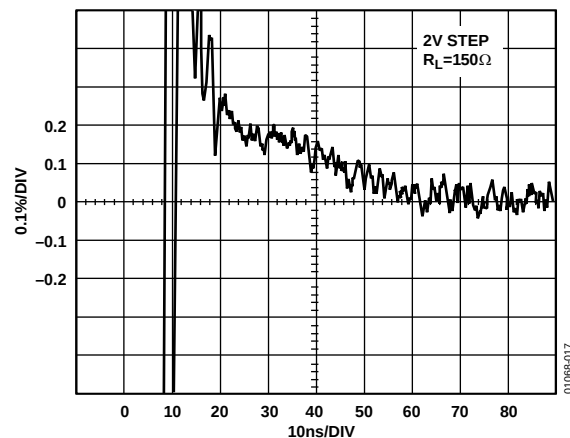
Figure 12. AD8108 Settling Time
