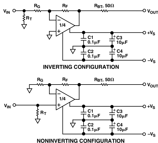
Figure 13. Inverting and Noninverting Configurations
