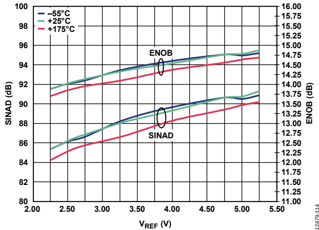
Figure 19. SINAD and ENOB vs. Reference Voltage ( V_{REF} ), MSOP
