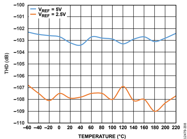
Figure 33. THD vs. Temperature, FLATPACK
