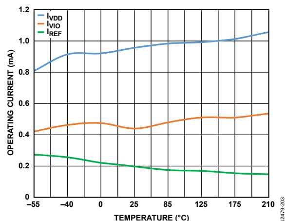
Figure 34. Operating Current vs. Temperature, FLATPACK
