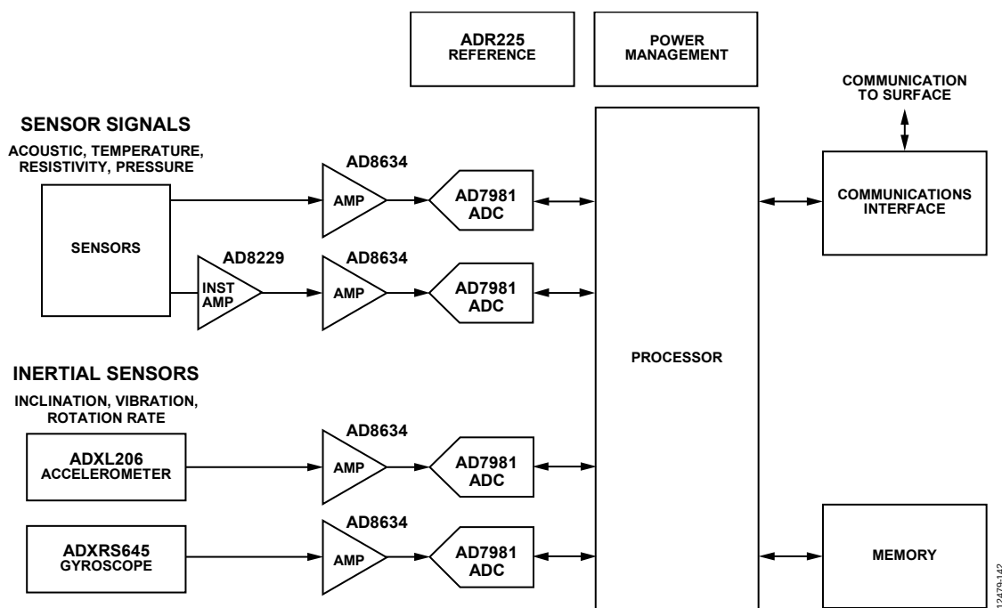
Figure 54. Simplified Data Acquisition System Signal Chain
