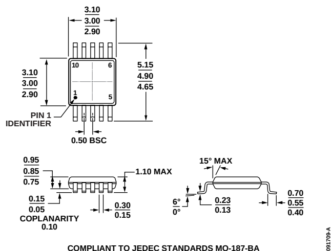
Figure 57. 10-Lead Mini Small Outline Package [MSOP] (RM-10)
