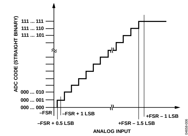
Figure 22. ADC Ideal Transfer Function
