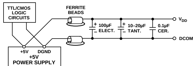
Figure 30. Differential LC Filter for Single +5 V Applications
