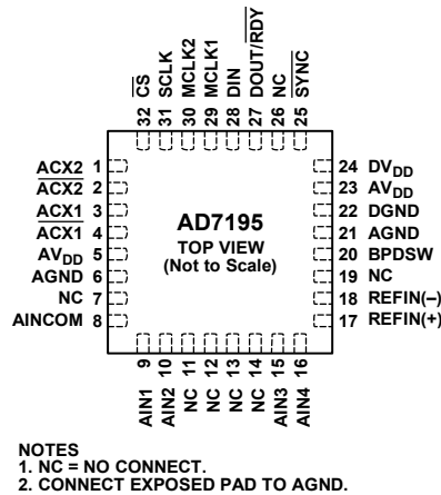
Figure 5. Pin Configuration
