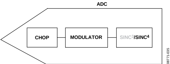
Figure 40. Chop Enabled
