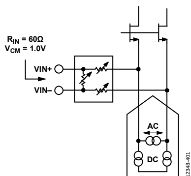
Figure 59. Equivalent Analog Input
