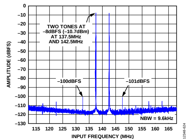
Figure 21. Two-Tone IMD Performance ( f_1 = 137.5 MHz, f_2 = 142.5 MHz)
