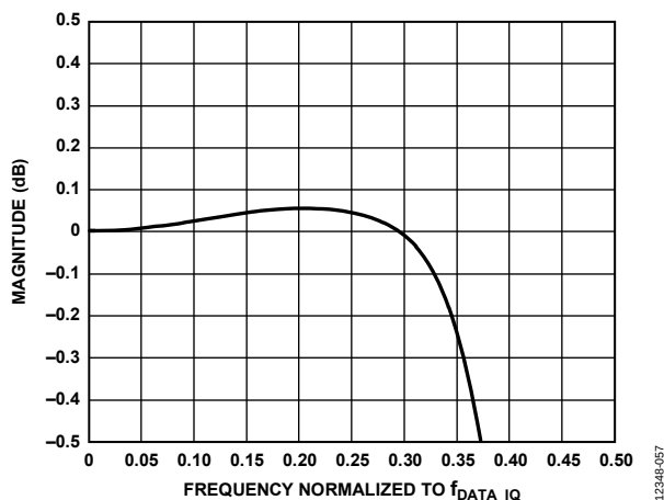
Figure 106. Pass Band Frequency Response of Decimate by 16
