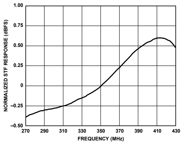
Figure 46. IF Pass Band Flatness (Includes Digital Filter)
