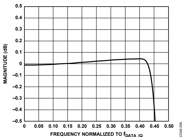
Figure 107. Pass Band Frequency Response of Decimate by 24
