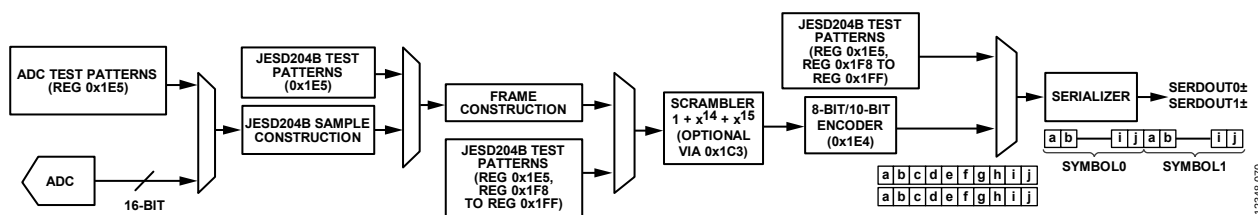
Figure 119. Digital Formatting of JESD204B Lanes
