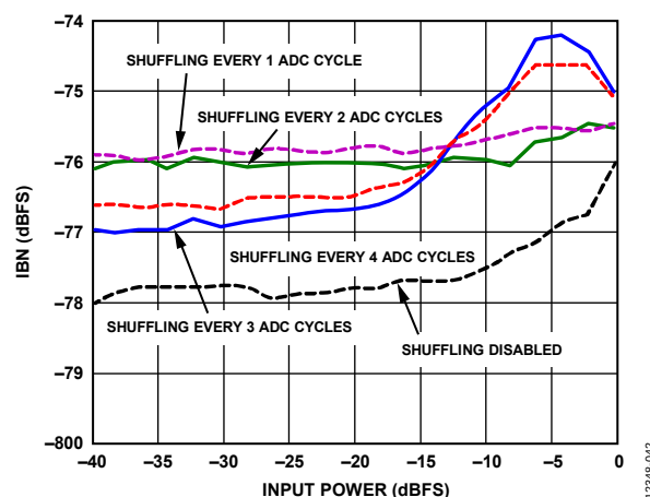
Figure 89. Pass Band Degradation in IBN (dBFS) as a Continuous Wave Tone at 225 MHz, Swept from -40 dBFS to -1 dBFS with Different Shuffling Rate Settings, Threshold Set to 0, F_{IF} = 180 MHz, BW = 80 MHz, F_{ADC} = 3.2 GHz, L_{EXT} = 43 nH
