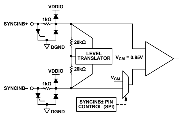
Figure 64. Equivalent SYNCIN± Input
