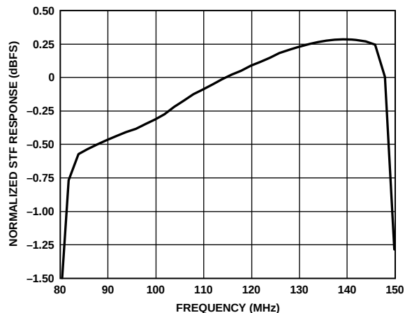
Figure 4. IF Pass Band Flatness (Includes Digital Filter)
