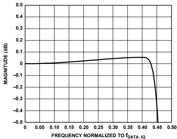
Figure 111. Pass Band Frequency Response of Decimate by 32
