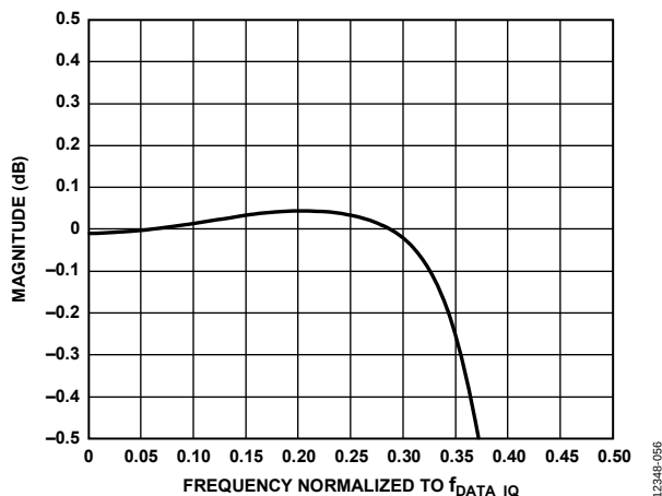
Figure 105. Pass Band Frequency Response of Decimate by 12
