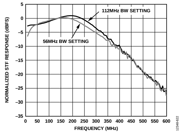
Figure 19. Wideband Frequency Response (Before Digital Filter)
