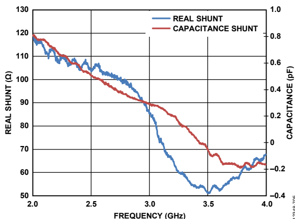
Figure 131. Equivalent Shunt Differential Input Impedance of the CLK \pm Pins with the Clock Synthesizer Disabled
