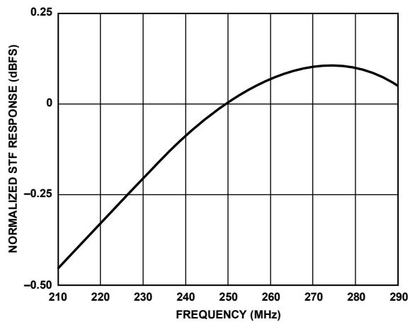
Figure 34. IF Pass Band Flatness (Includes Digital Filter)
