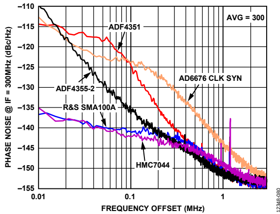
Figure 135. Close In Phase Noise Comparison for Different Analog Devices Clock Sources when Compared to the R&S SMA100A and the AD6676 Clock Synthesizer (IF = 300 MHz, BW = 40 MHz, F_{ADC} = 3.2 GHz, L = 19 nH)
