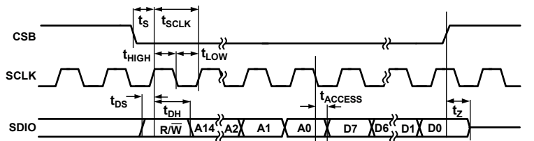
Figure 149. SPI 3-Wire Read Operation Timing
