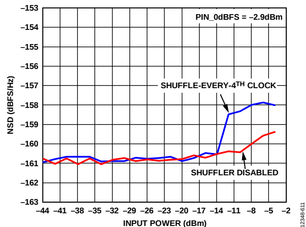
Figure 8. NSD vs. CW Input Power, CW at 108 MHz (NSD Measured at IF Center of 115 MHz)
