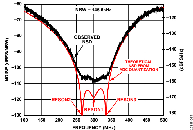
Figure 71. Measured vs. Ideal NTF ( F_{IF} = 300 MHz, BW = 80 MHz, F_{ADC} = 3.2 GHz, L_{EXT} = 19 nH)
