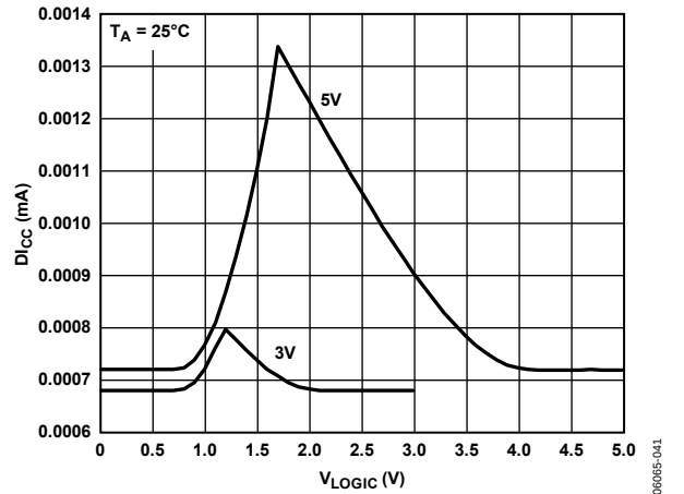
Figure 24. D_{ICC} vs. Logic Input Voltage
