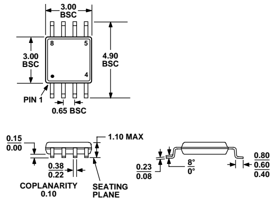
Figure 40. 8-Lead Mini Small Outline Package [MSOP]
