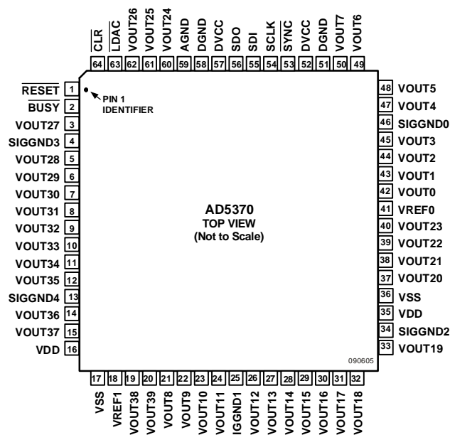
Figure 6.64-Lead LQFP Pin Configuration
