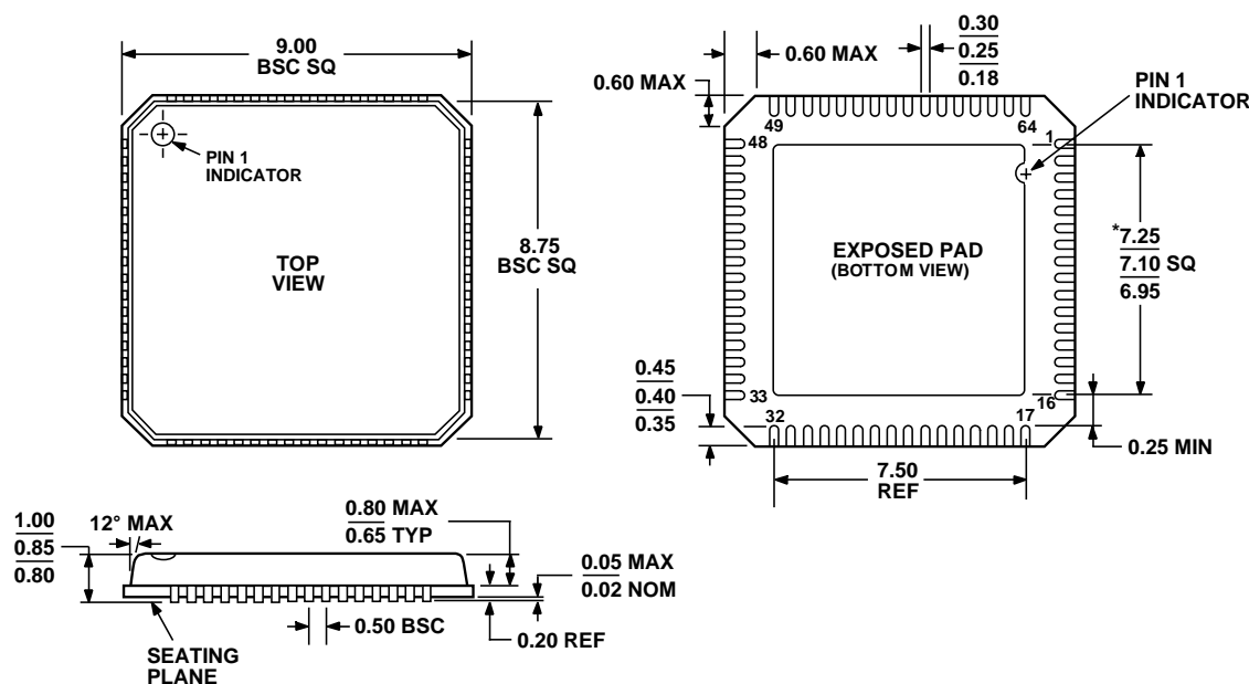
Figure 14. 64-Lead Free Chip Scale Package [LFCSP] (CP-64-3)
