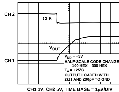
Figure 16. Half-Scale Settling Time
