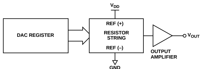
Figure 20. DAC Architecture
