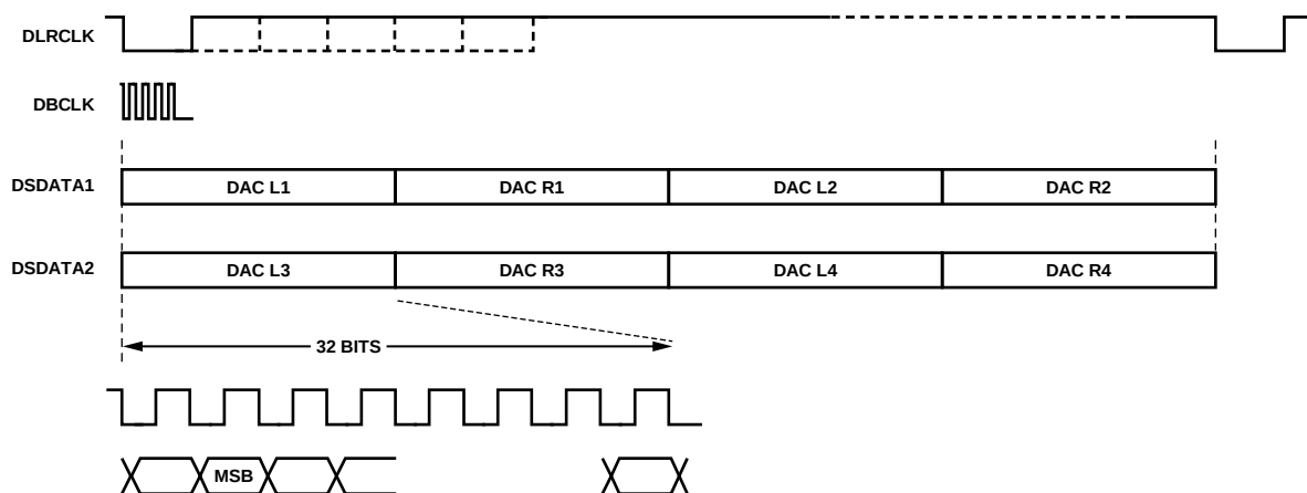
Figure 14. Dual-Line, DAC TDM Mode (Applicable to 192 kHz Sample Rate, 8-Channel Mode)
