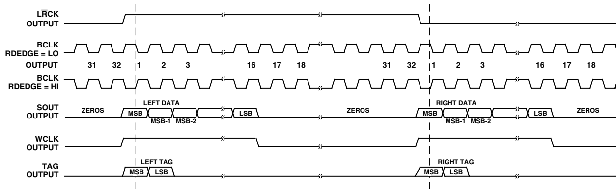
Figure 13. Serial Data Output Timing: Master Mode, Left-Justified with No MSB Delay, \overline{S\text{M}} = \text{LO} , \overline{R\text{LJUST}} = \text{LO} , \overline{\text{MSBDLY}} = \text{HI}
