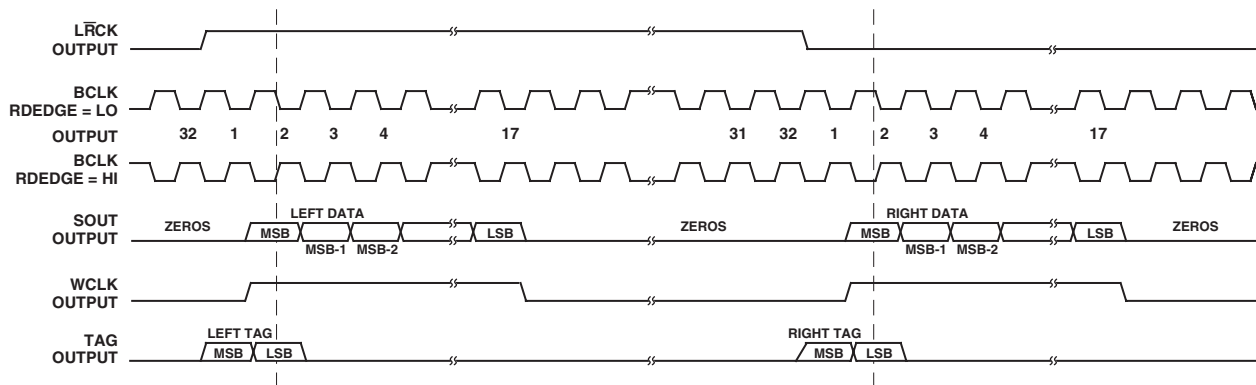
Figure 14. Serial Data Output Timing: Master Mode, I 2 S-Justified, \overline{S\text{M}} = \text{LO} , \overline{R\text{LJUST}} = \text{LO} , \overline{\text{MSBDLY}} = \text{LO}
