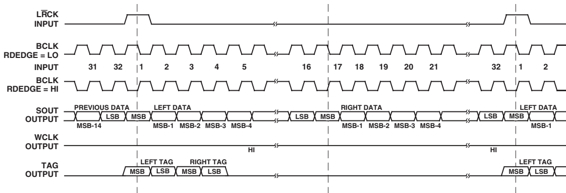
Figure 15. Serial Data Output Timing: Slave Mode, Left-Justified with No MSB Delay, 32-Bit Frame Mode, \overline{S\text{M}} = \text{HI} , \overline{R\text{LJUST}} = \text{LO} , \overline{\text{MSBDLY}} = \text{HI}
