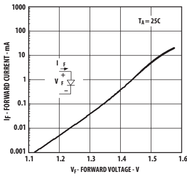
Figure 11. Typical input diode forward characteristics.
