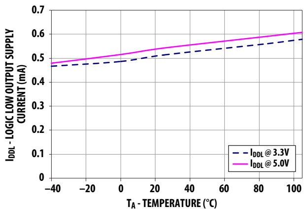
Figure 11 Logic Low Output Supply Current vs. Temperature
