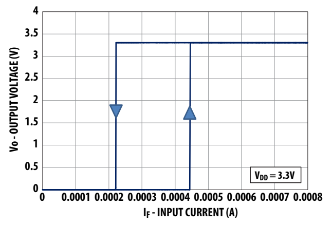
Figure 15 Output Voltage vs. Input Current @ V_{DD} = 3.3V
