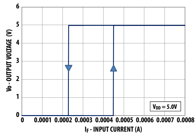
Figure 16 Output Voltage vs. Input Current @ V_{DD} = 5V
