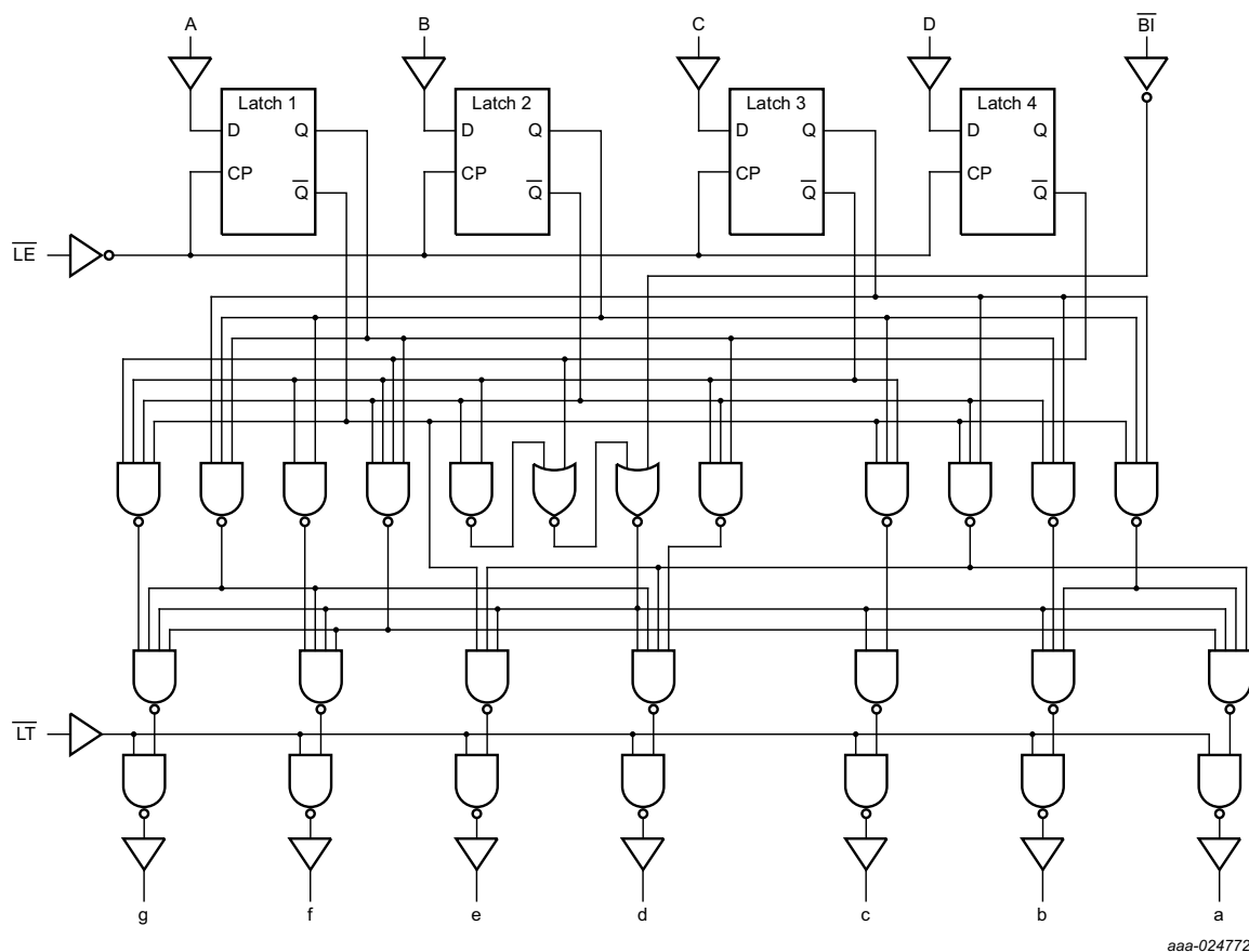
Fig 4. Logic diagram
