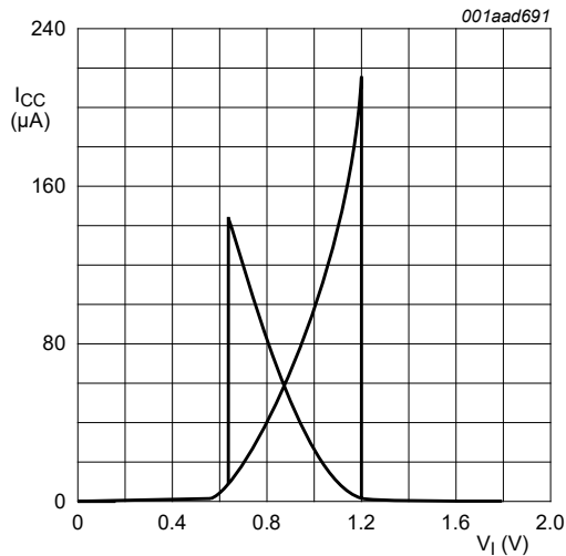
Fig. 9. Typical transfer characteristics; V_{CC} = 1.8 \text{ V}
