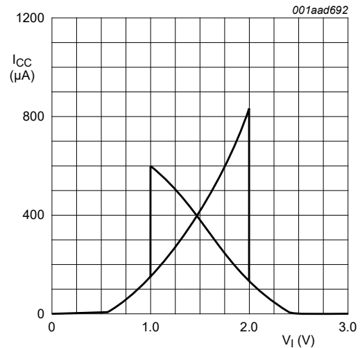
Fig. 10. Typical transfer characteristics; V_{CC} = 3.0 \text{ V}
