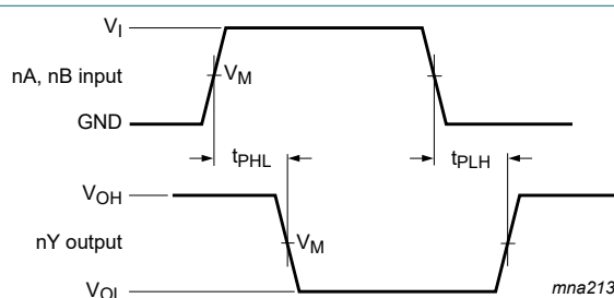
Fig. 6. The data input (nA, nB) to output (nY) propagation delays
