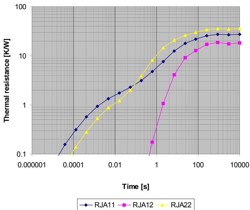
Figure 20. Transient Thermal 1W Step Response; Device on 2s2p JEDEC Standard Thermal Test Board
