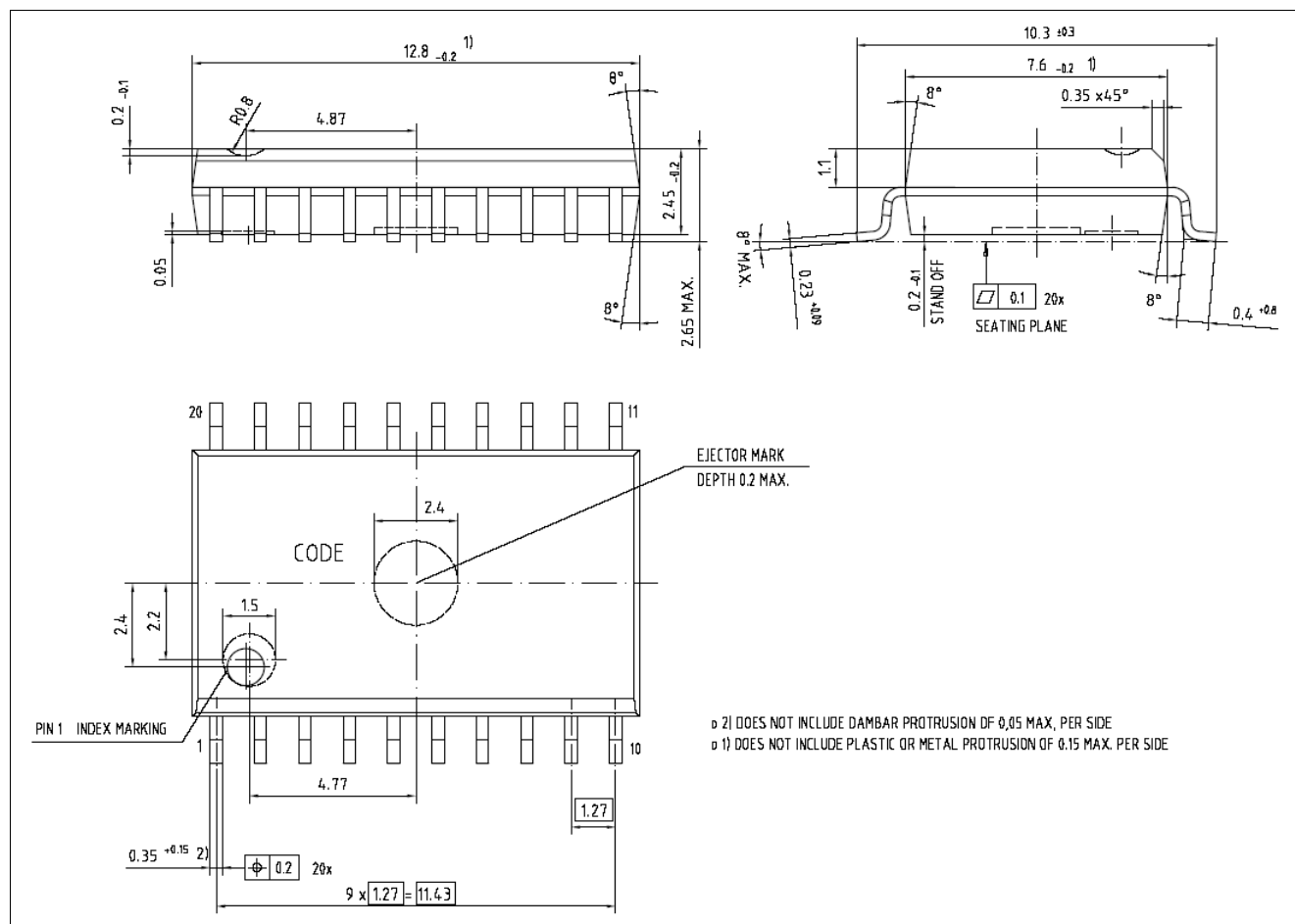
Figure 9: PG-DSO-20-55 (Plastic Dual Small Outline Package)
