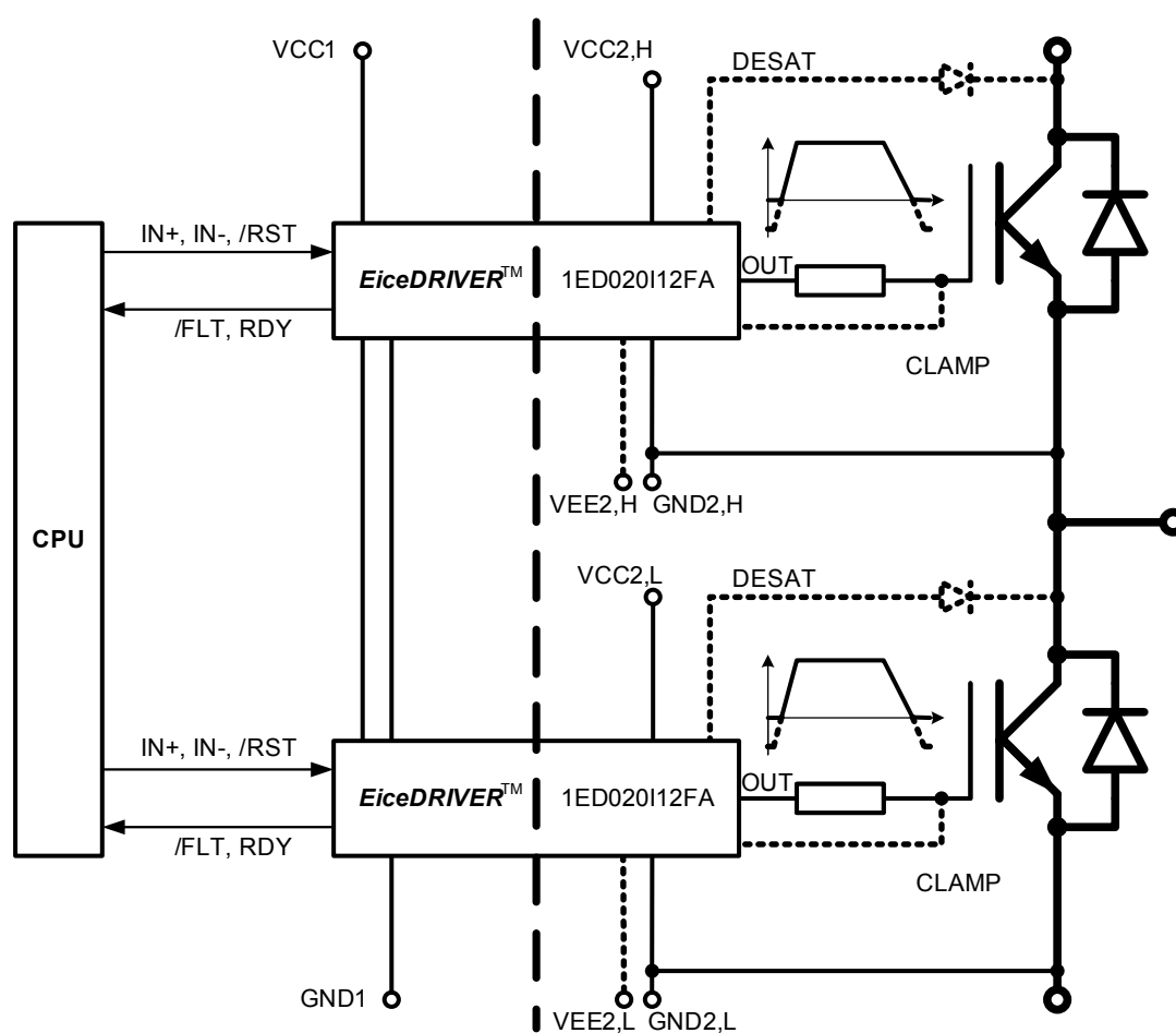
Figure 1: Typical Application
